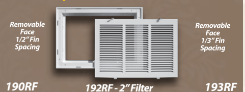
Fixed Bar Type Return Air Grille
